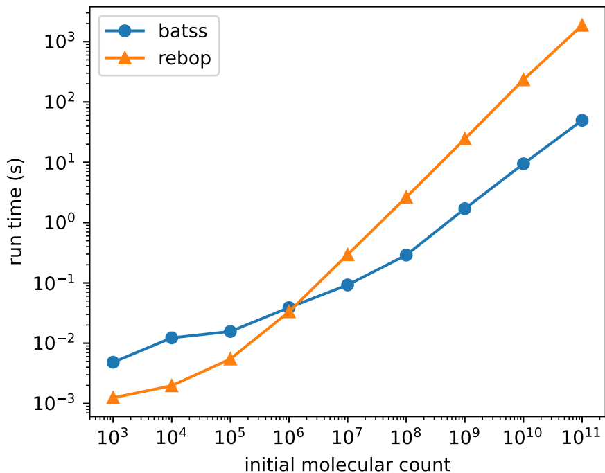
Lotka Volterra: run time to simulate t=1.0
